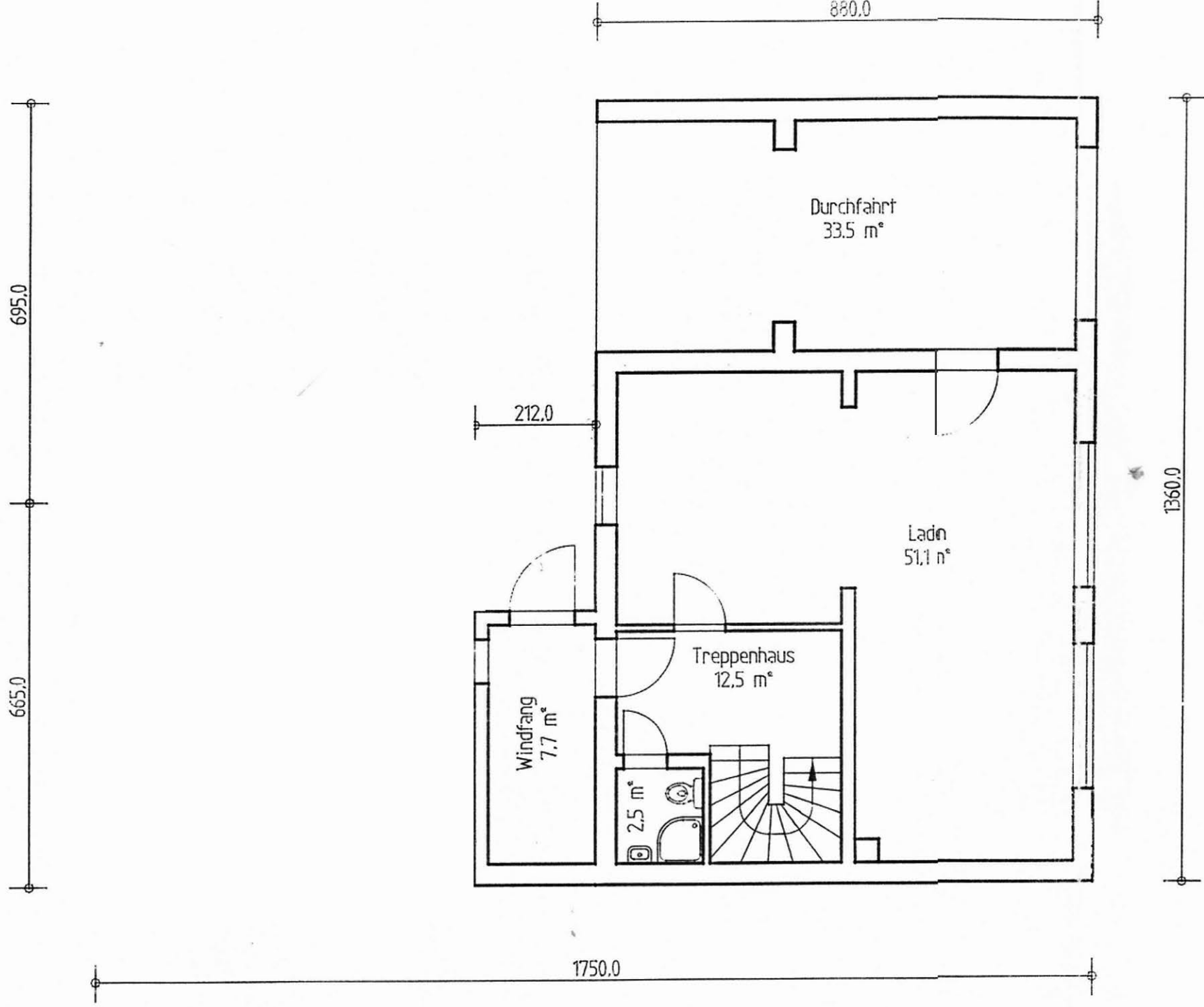
Grundriß Erdgeschoß
