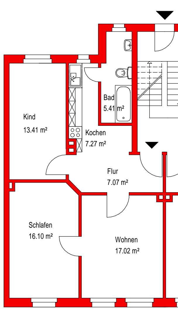
Erdgeschoss - Links
