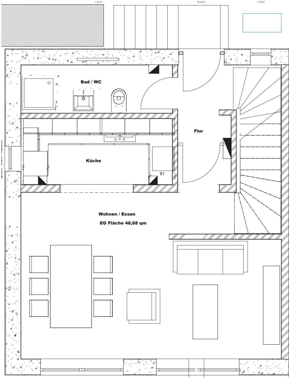
ERDGESCHOß LAYOUT
