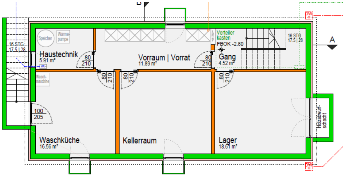
Plan UG
