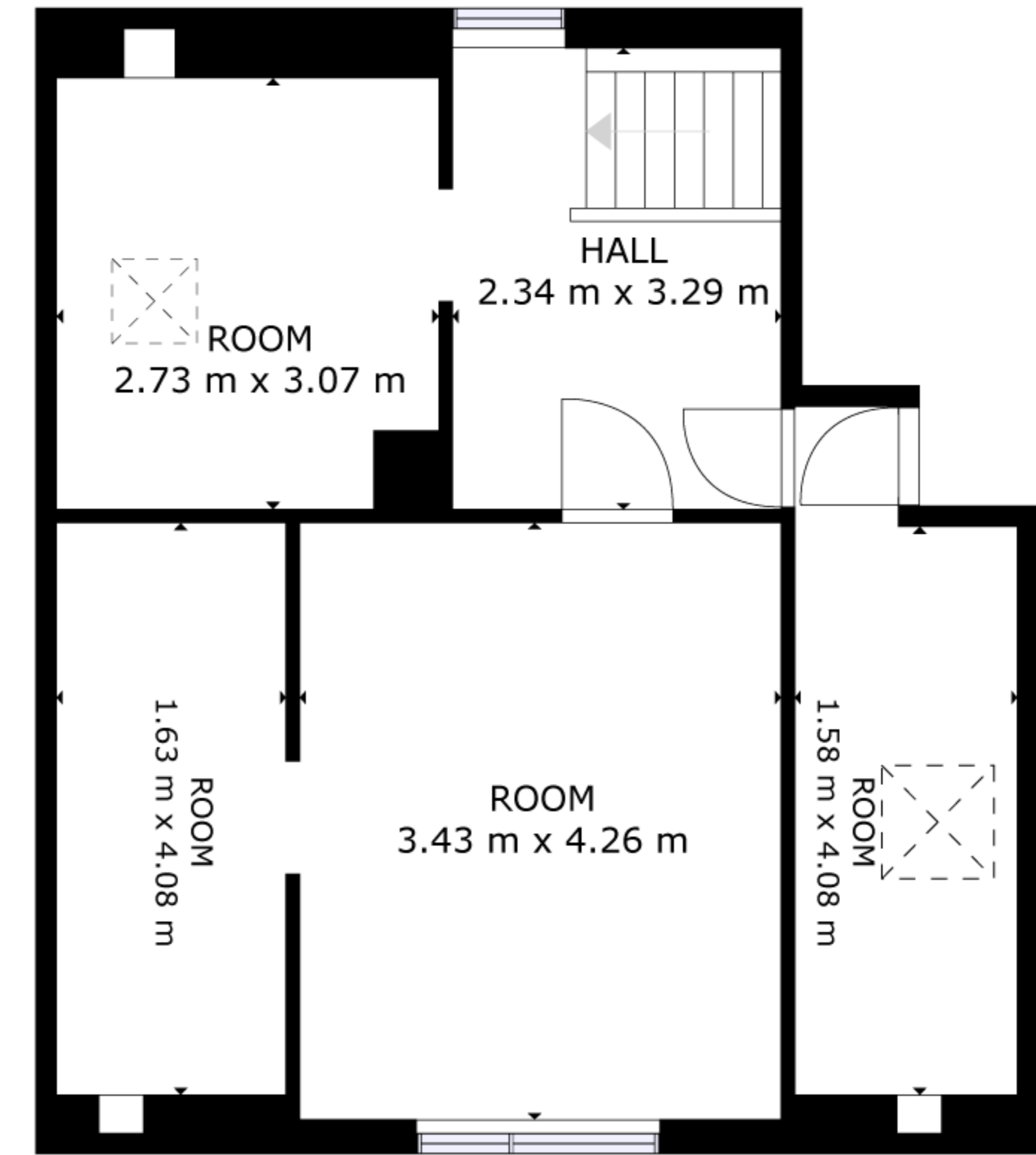
FLOOR 2
