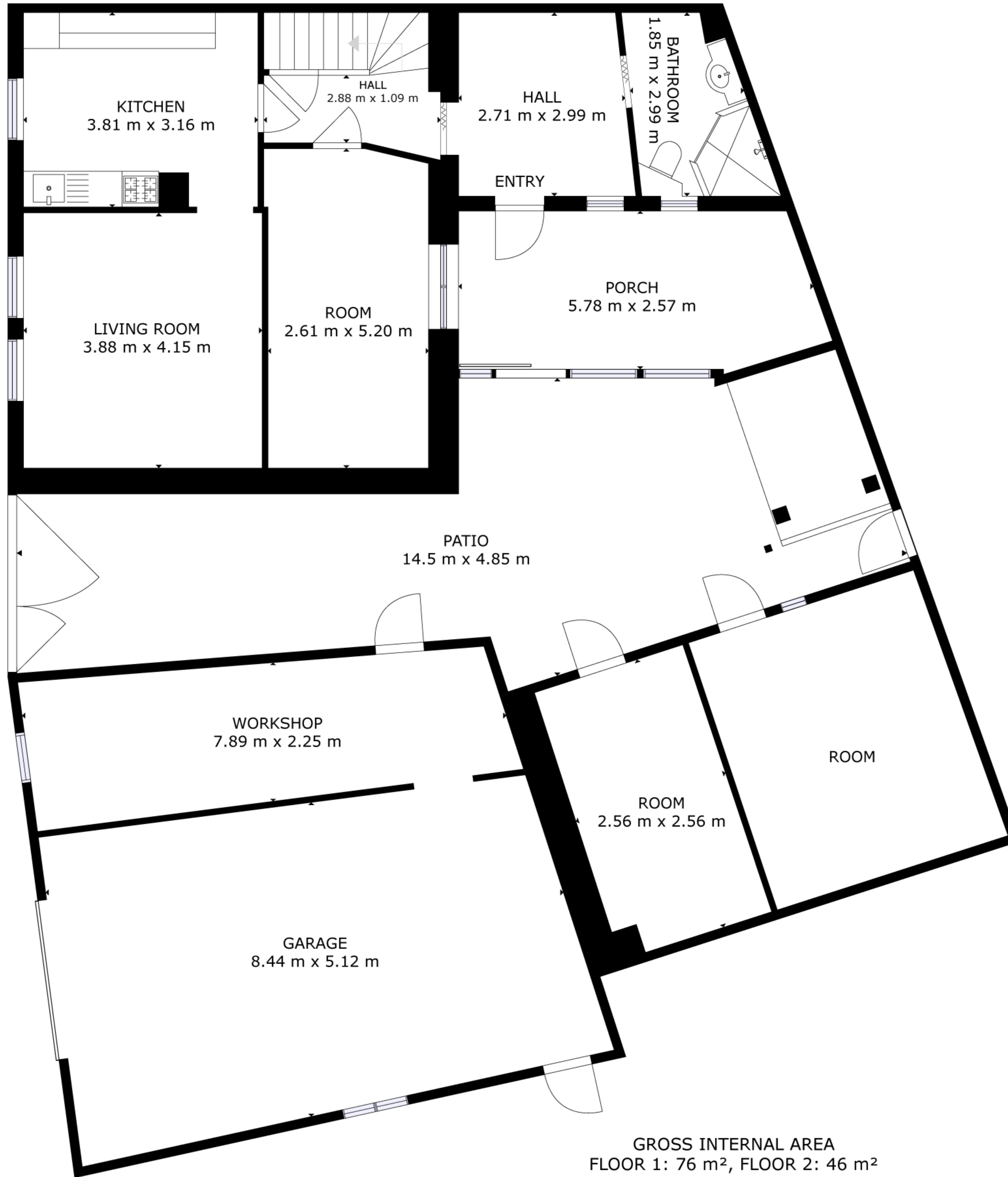
FLOOR 1
