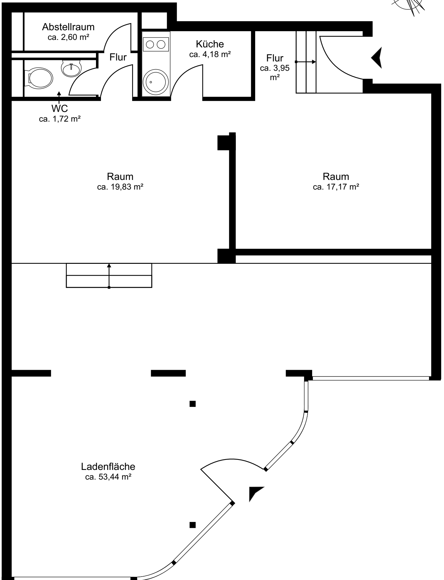
Erdgeschoss links
