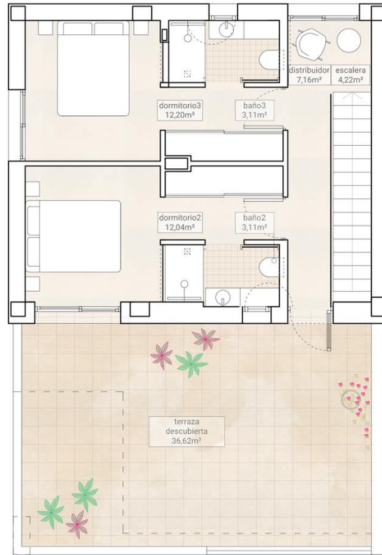
PLANTA PRIMERA/FIRST FLOOR Superficies útiles/Useful surfaces
