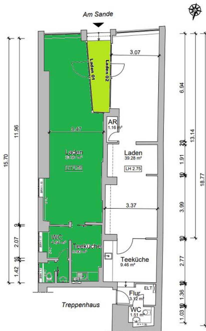
Grundriß Erdgeschoß
