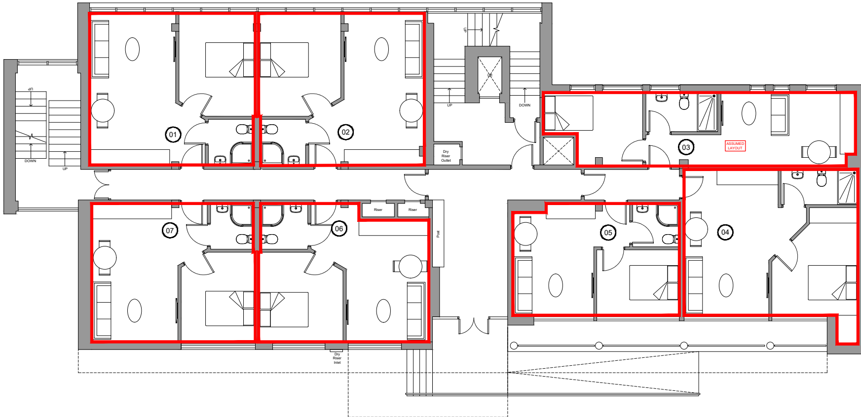
Proposed Ground Floor Plan Scale 1:100
