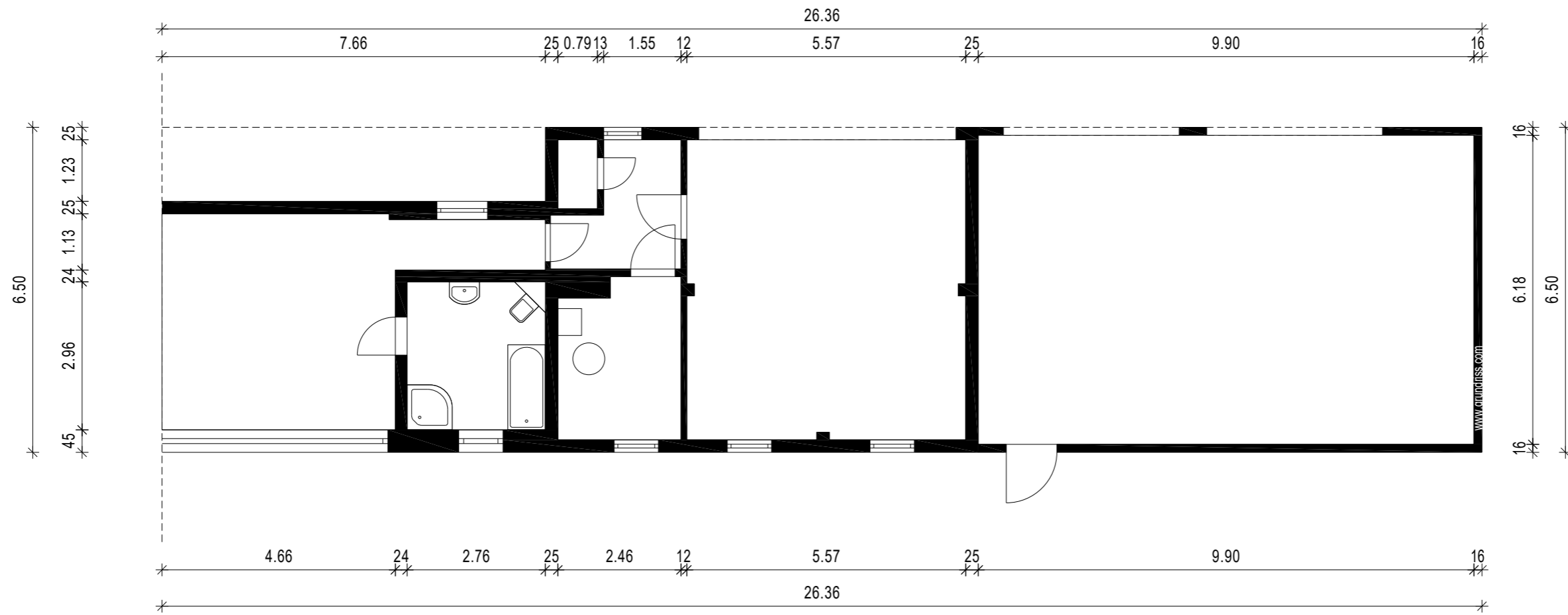
Erdgeschoss 2-2
