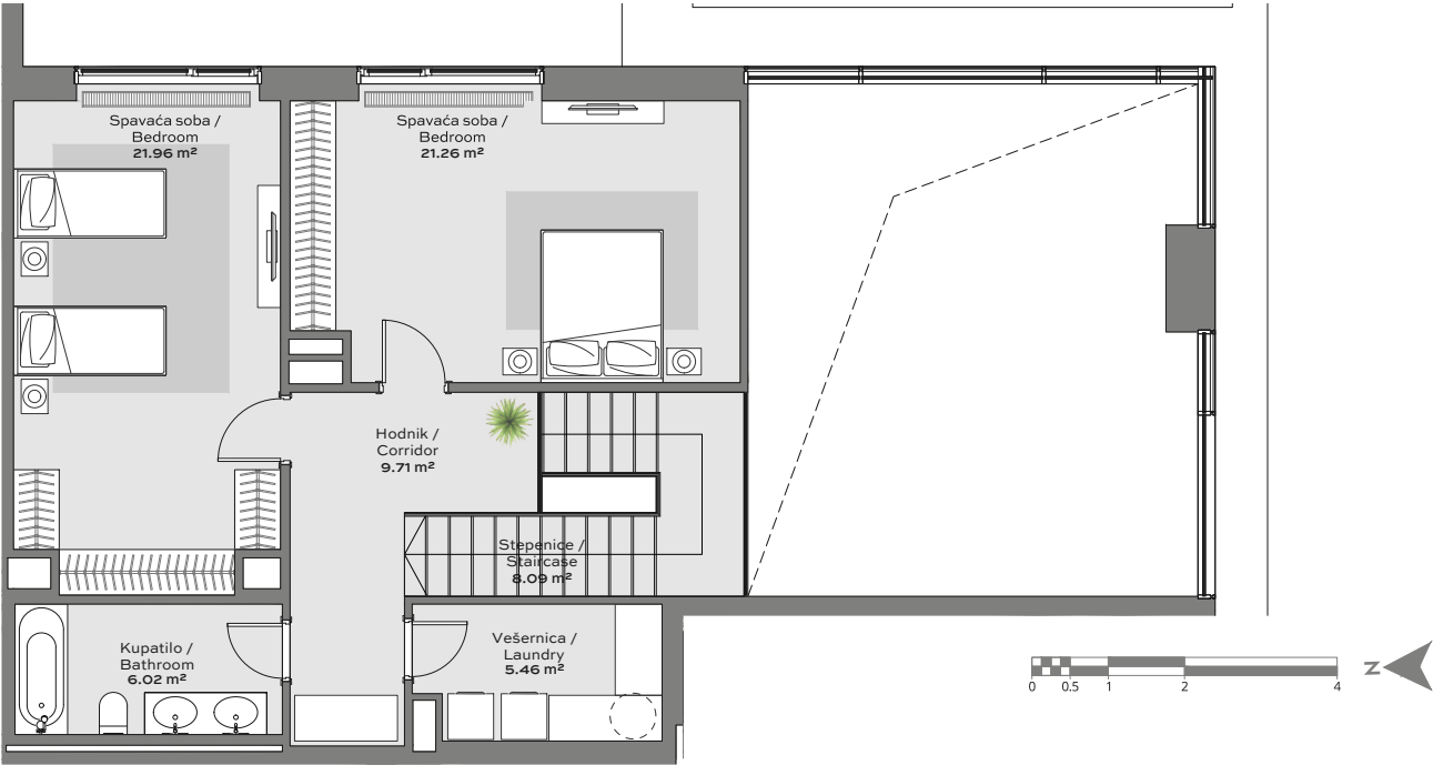
LEVEL PLAN - FLOOR NO. 24 RIVER
