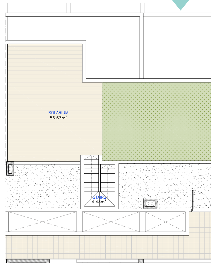
ROOF FLOOR
