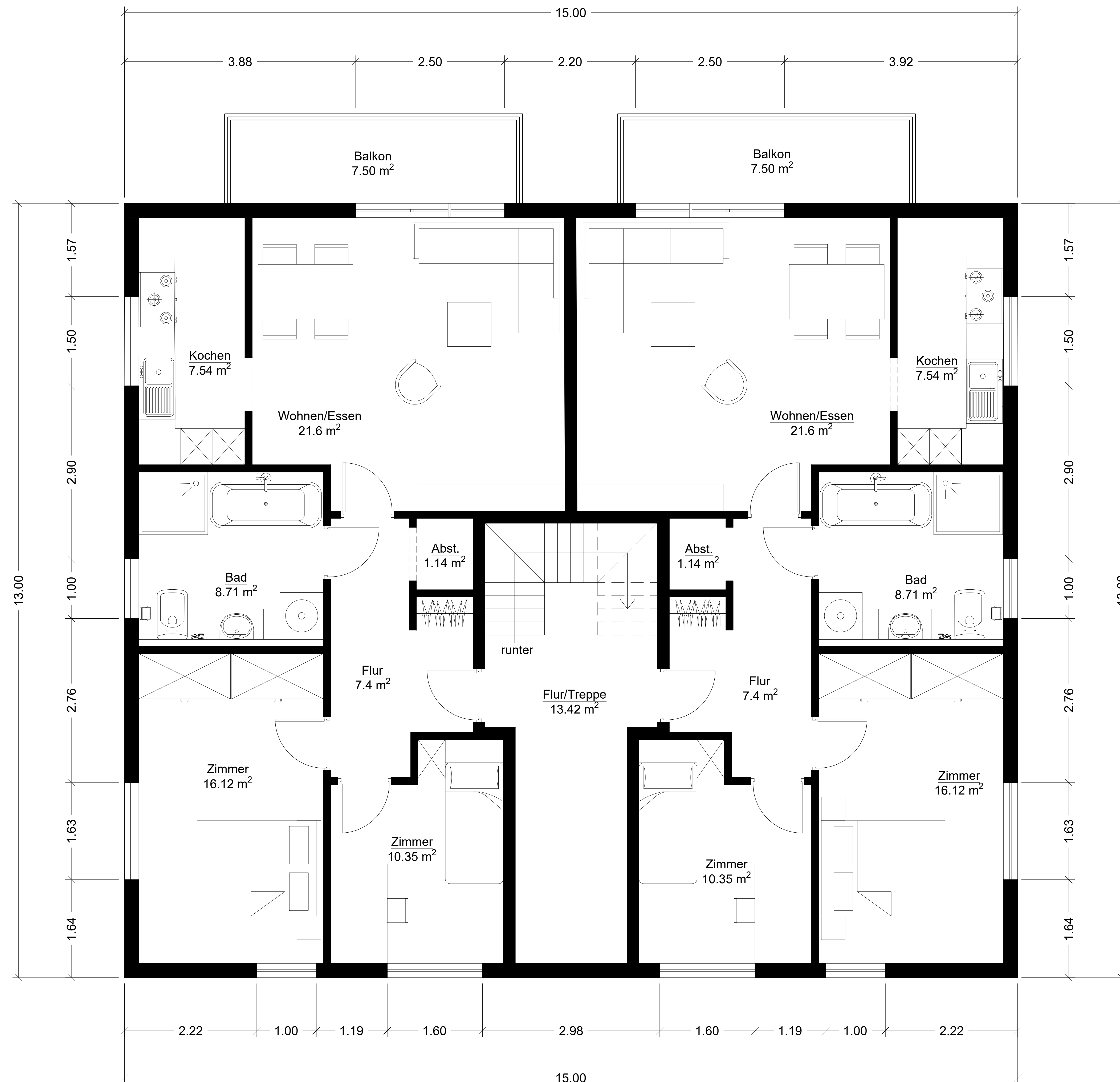
ATTIC FLOOR PLAN
