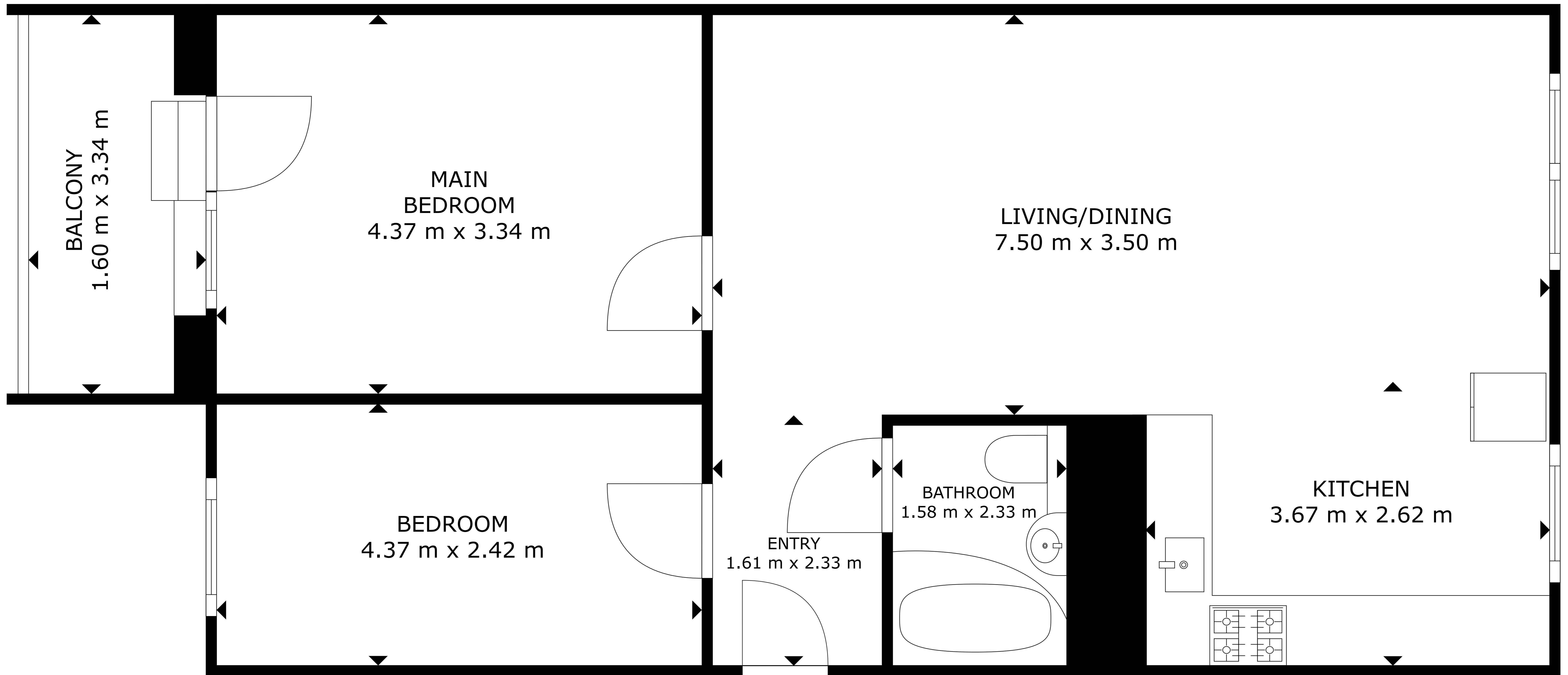
FLOOR PLAN
