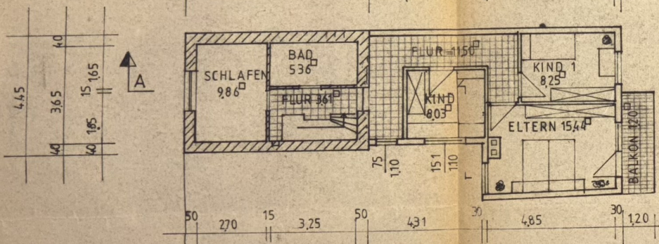
-OBERGESCHOSS-
