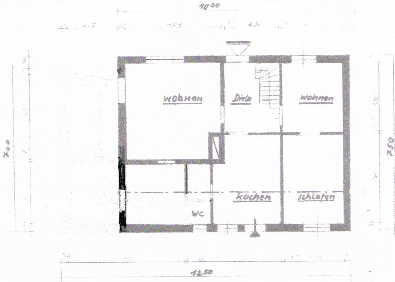
Erdgeschoss.
