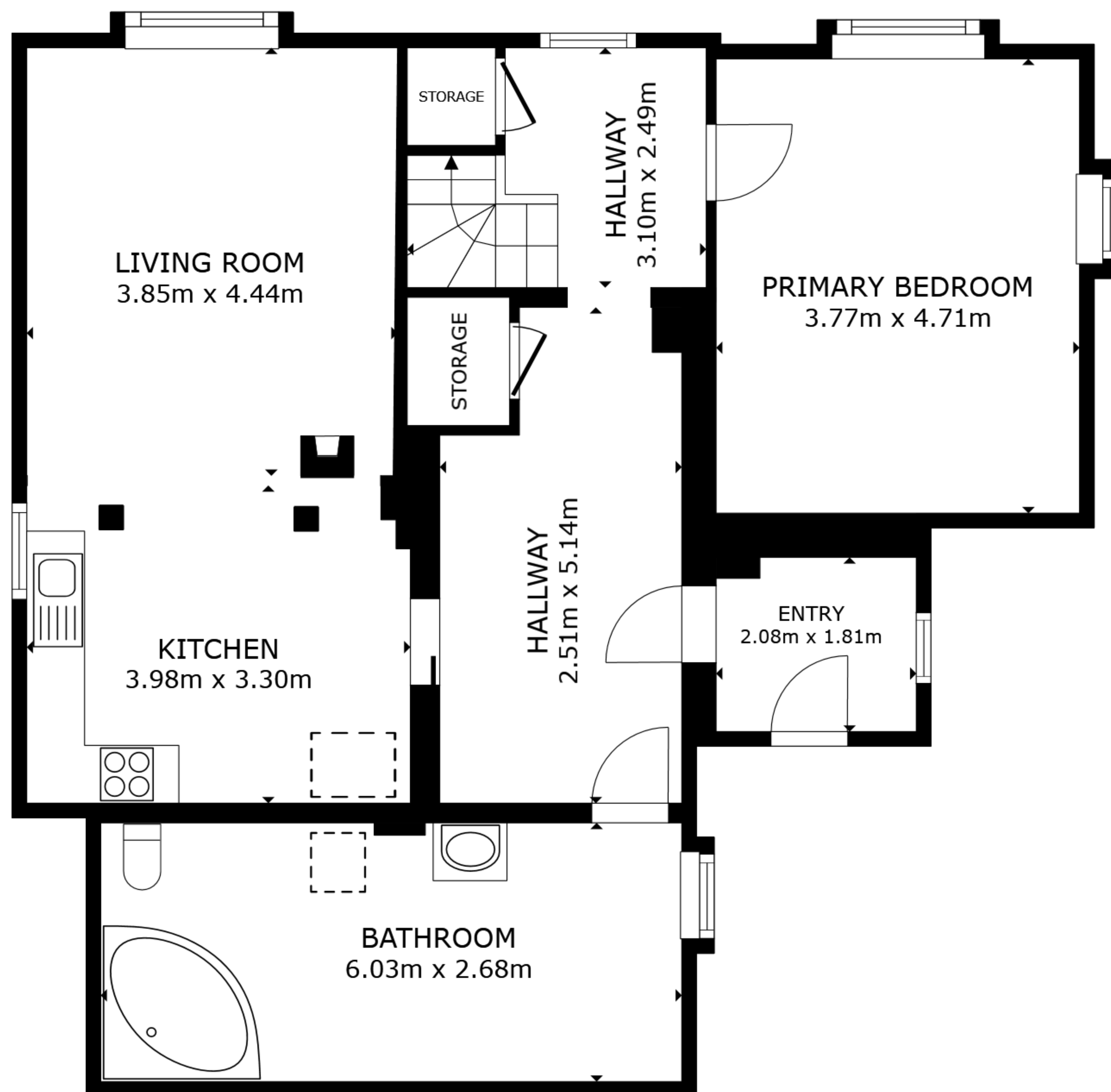
FLOOR 1
