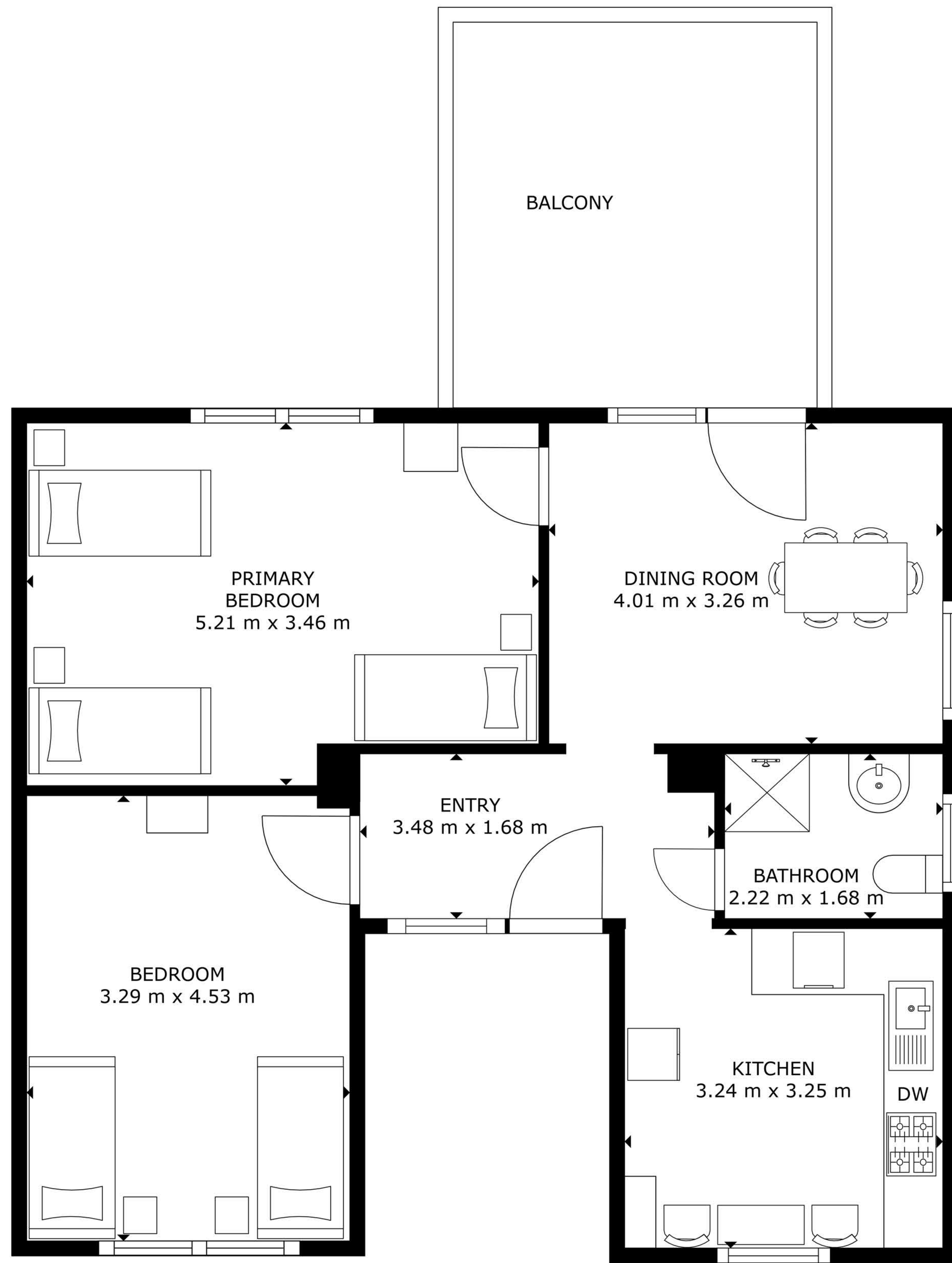
FLOOR PLAN
