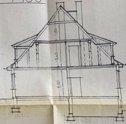
Cross-section 1-6
