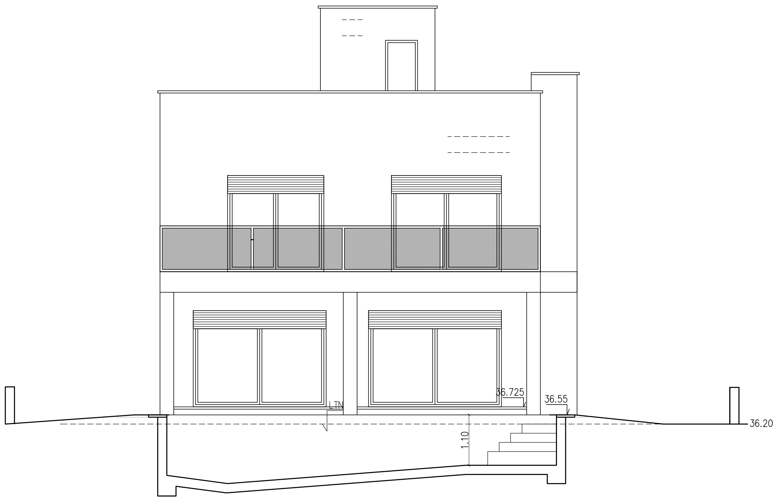
FACHADA PRINCIPAL
