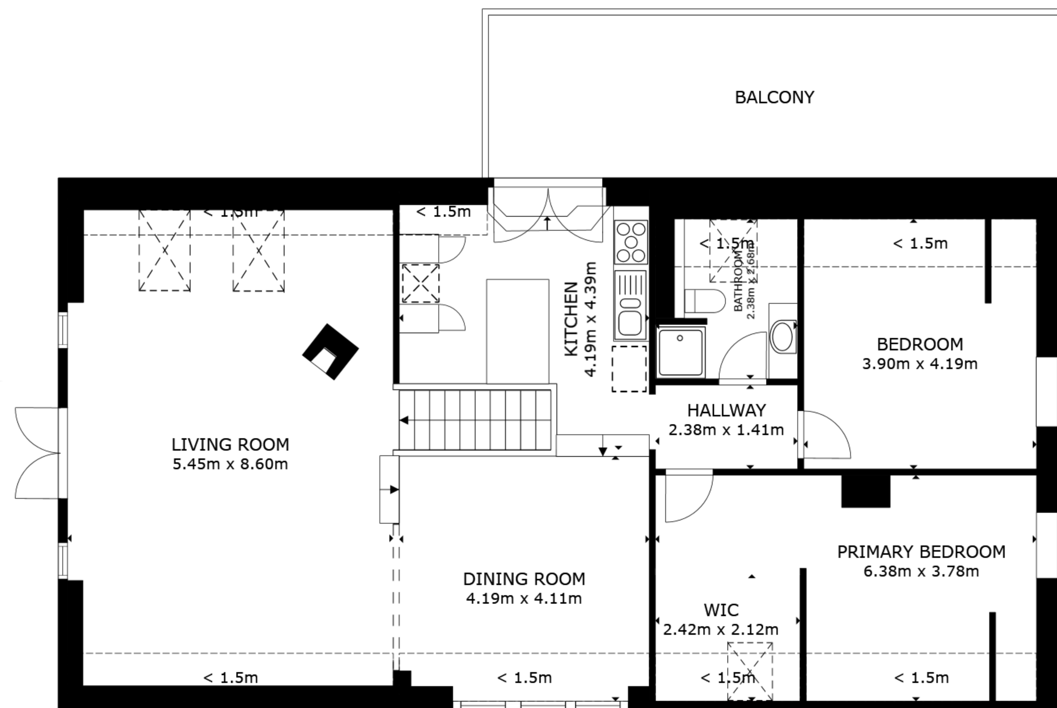
FLOOR 1
