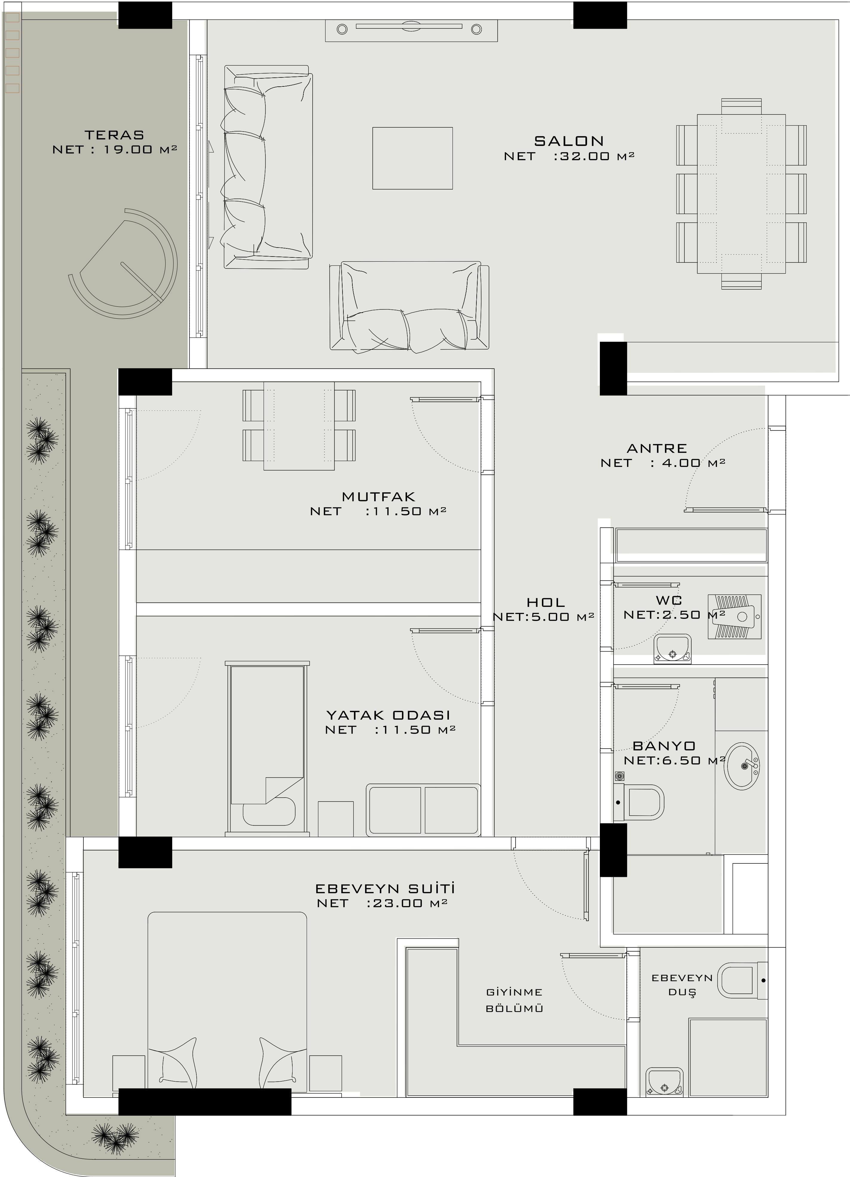
DAİRE PLANI
