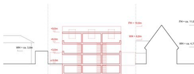
Schnitt Ost-West
