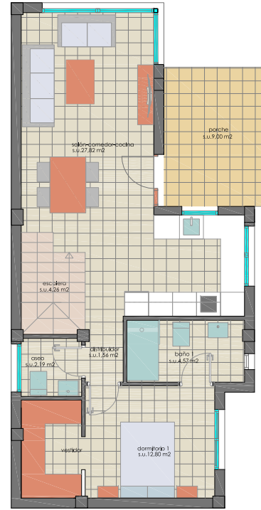
PLANTA BAJA GROUND FLOOR
