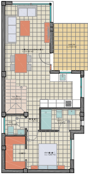
PLANTA BAJA GROUND FLOOR
