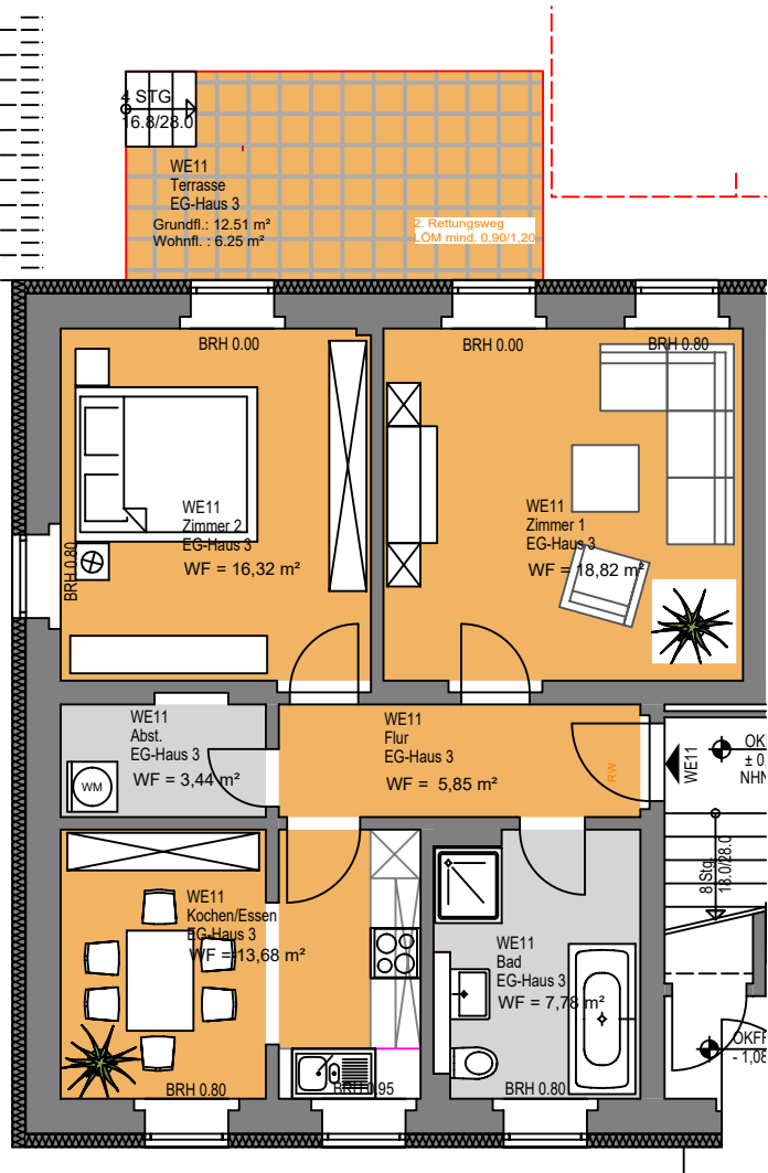
Erdgeschoss WE11
