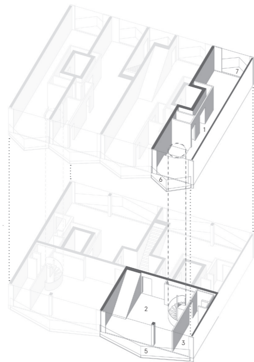
ISOMETRIE | ISOMETRY
