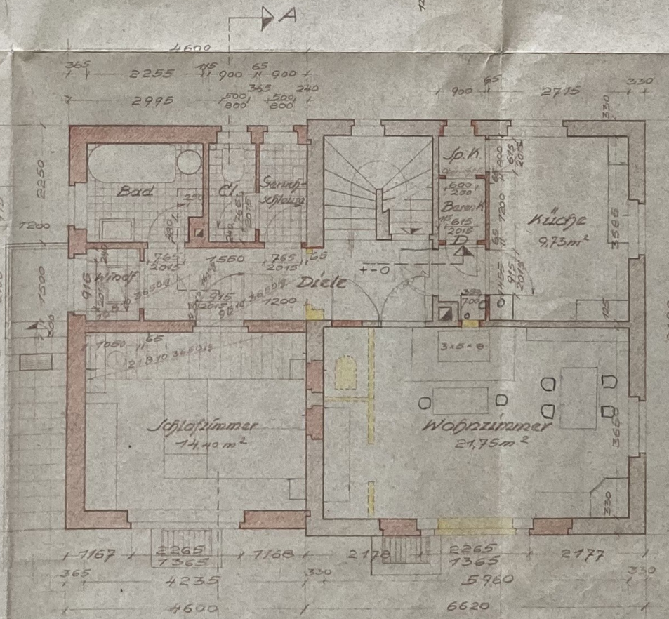
Erdgeschloß
