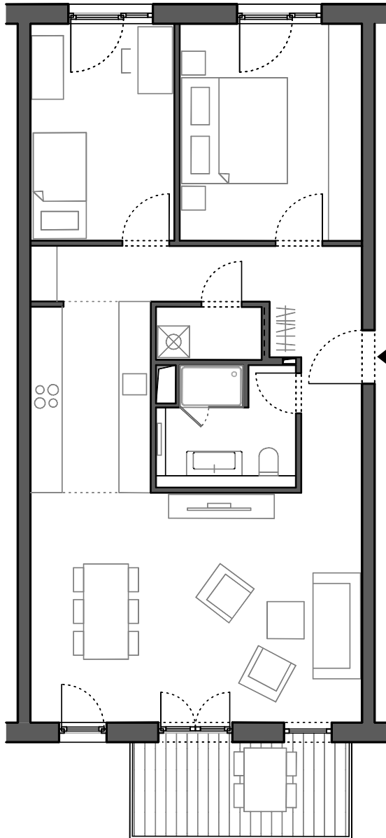
Grundriss M 1-100: WE 02; 04
