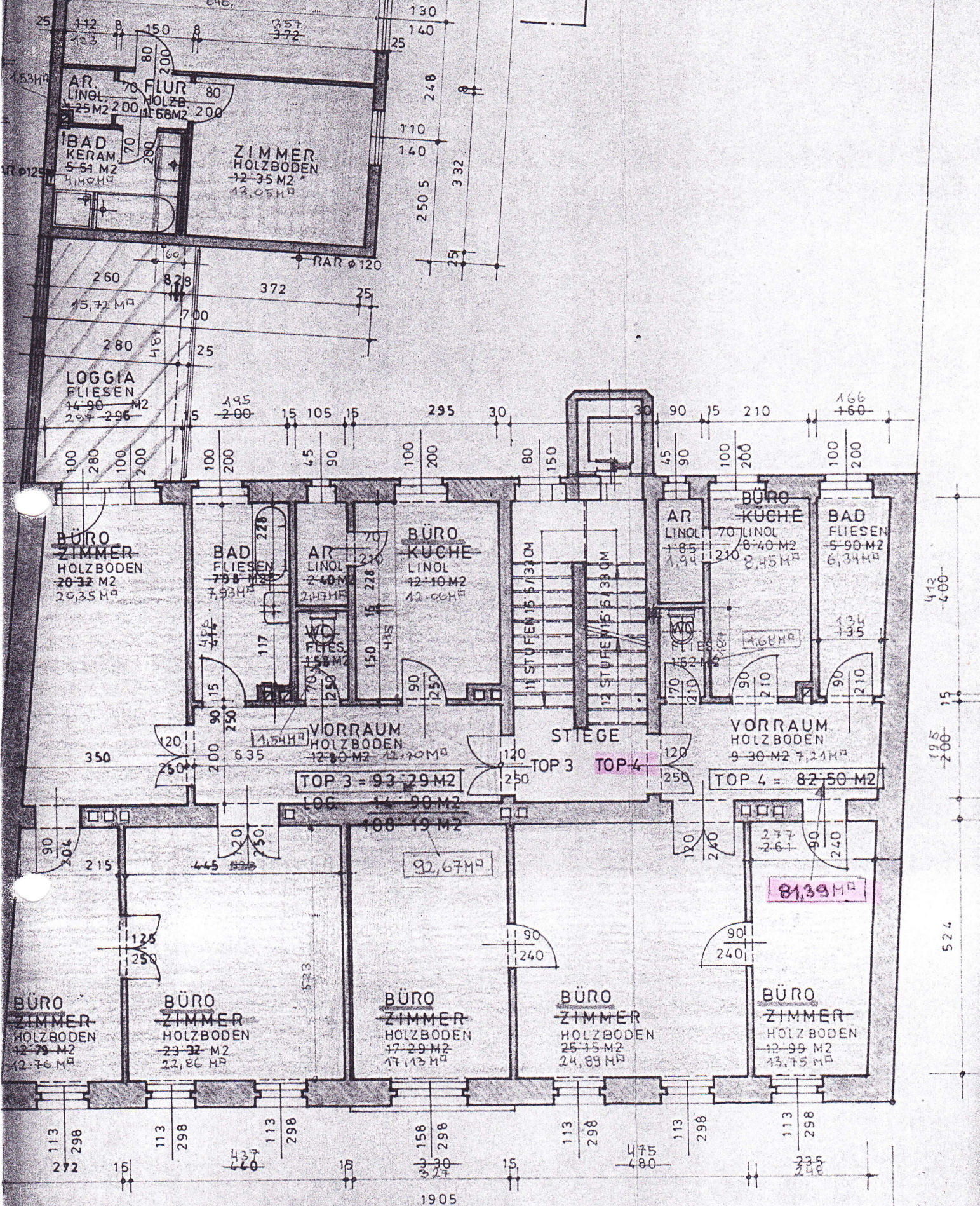
GRUNDRISS 1. STOCK
