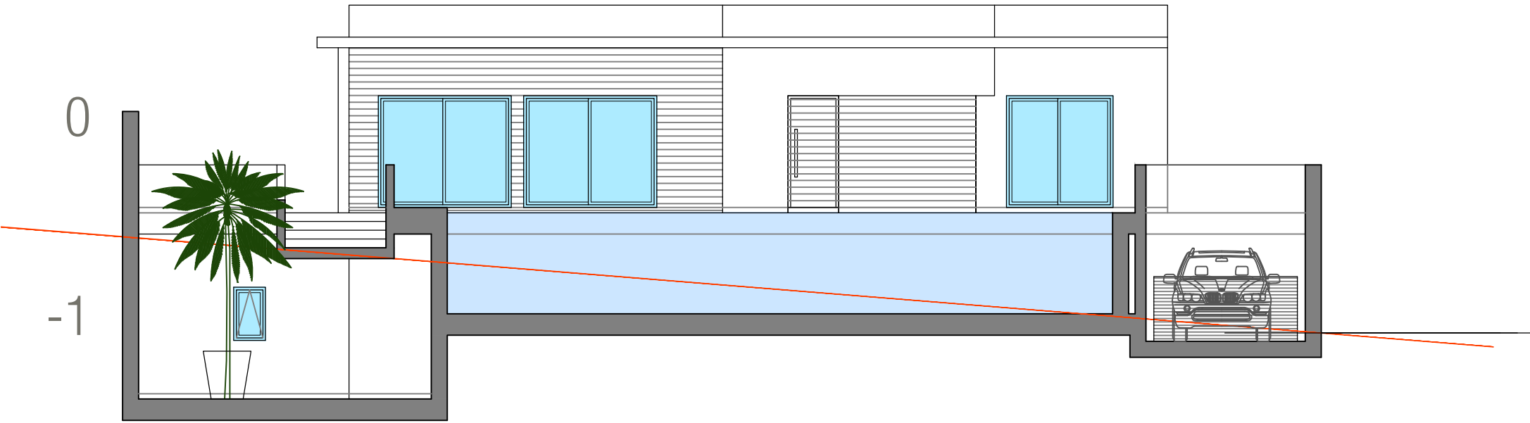
Façade A
