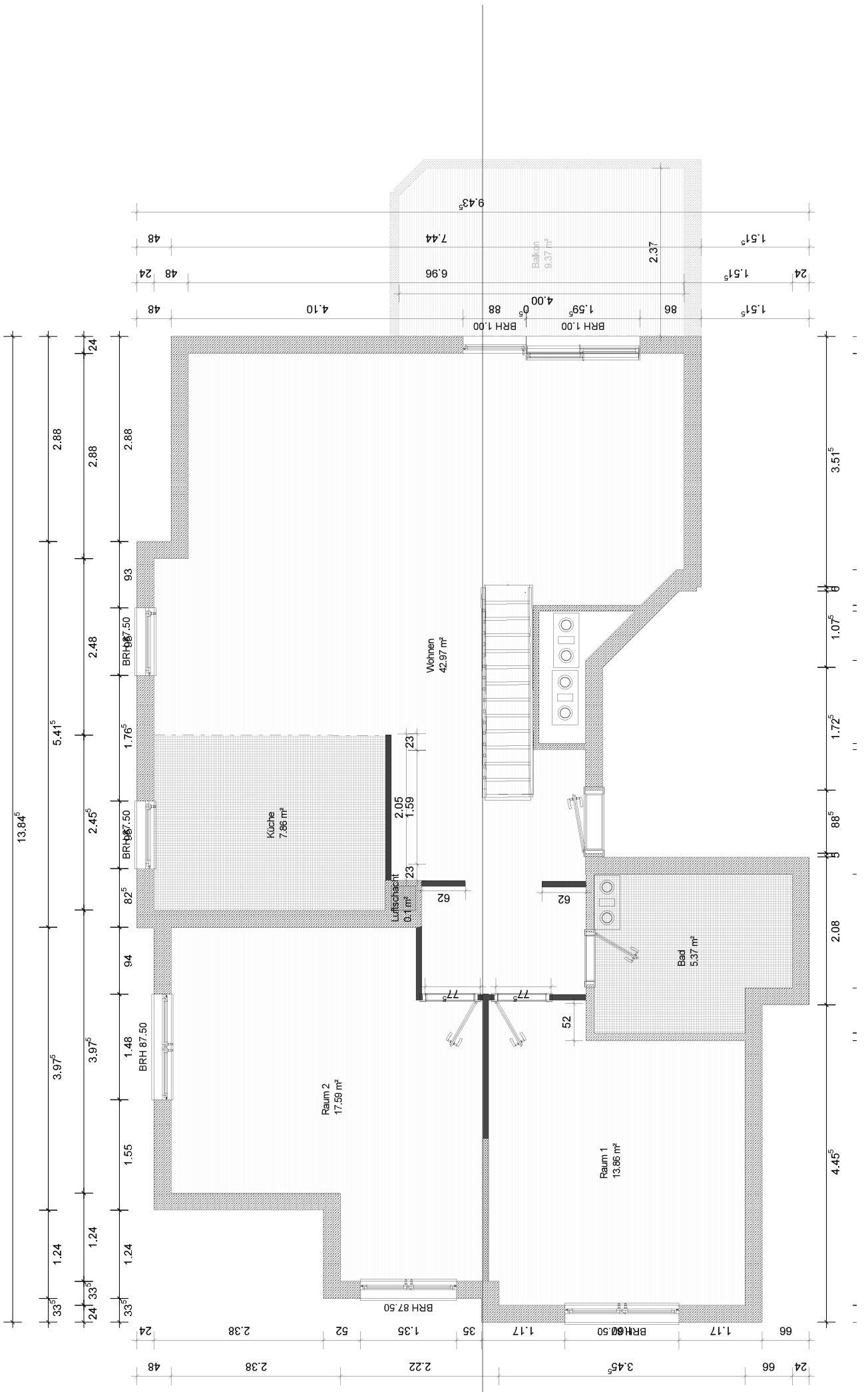
Architectural floor plan showing room layouts, dimensions, and area calculations for a residential unit. The plan includes labels for rooms such as Wohnen (Living Area), Küche (Kitchen), Wuschlraum (Washroom), Bad (Bathroom), Balkon (Balcony), Raum 1, and Raum 2, along with their respective areas in square meters. Dimensions are provided in meters and millimeters throughout the drawing.
