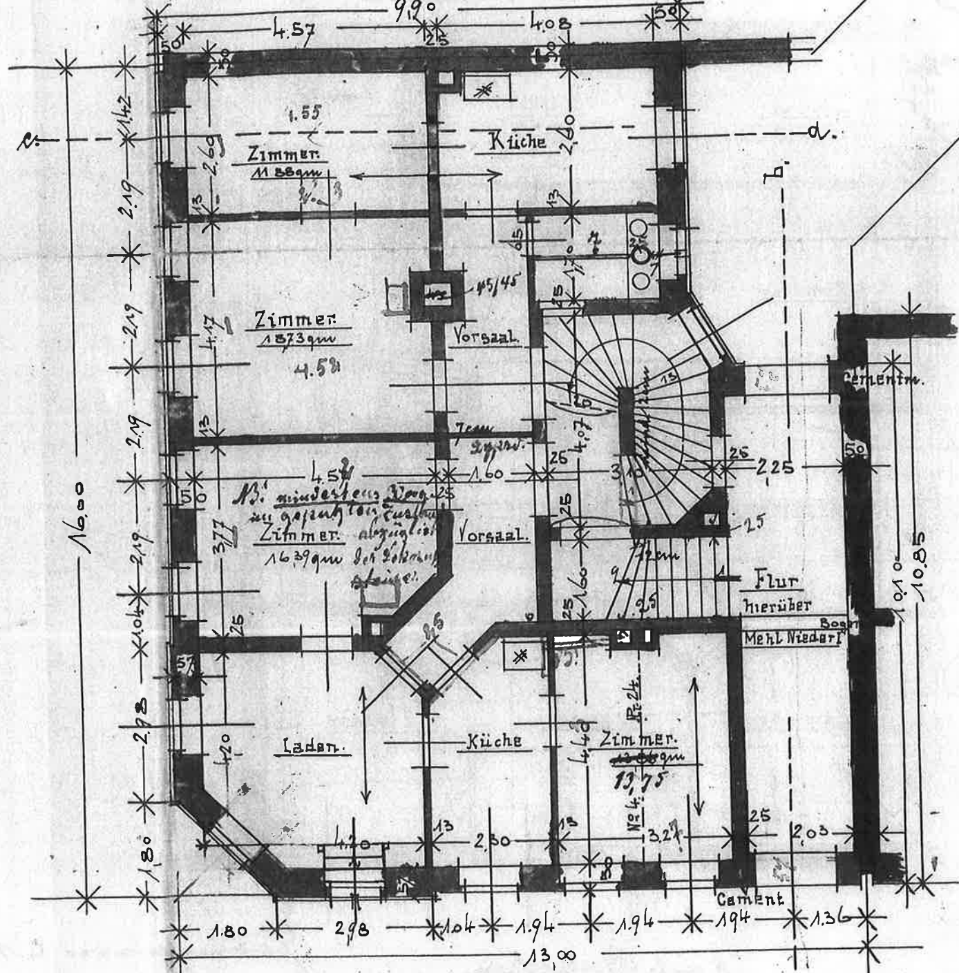
Erdergeschoss.
