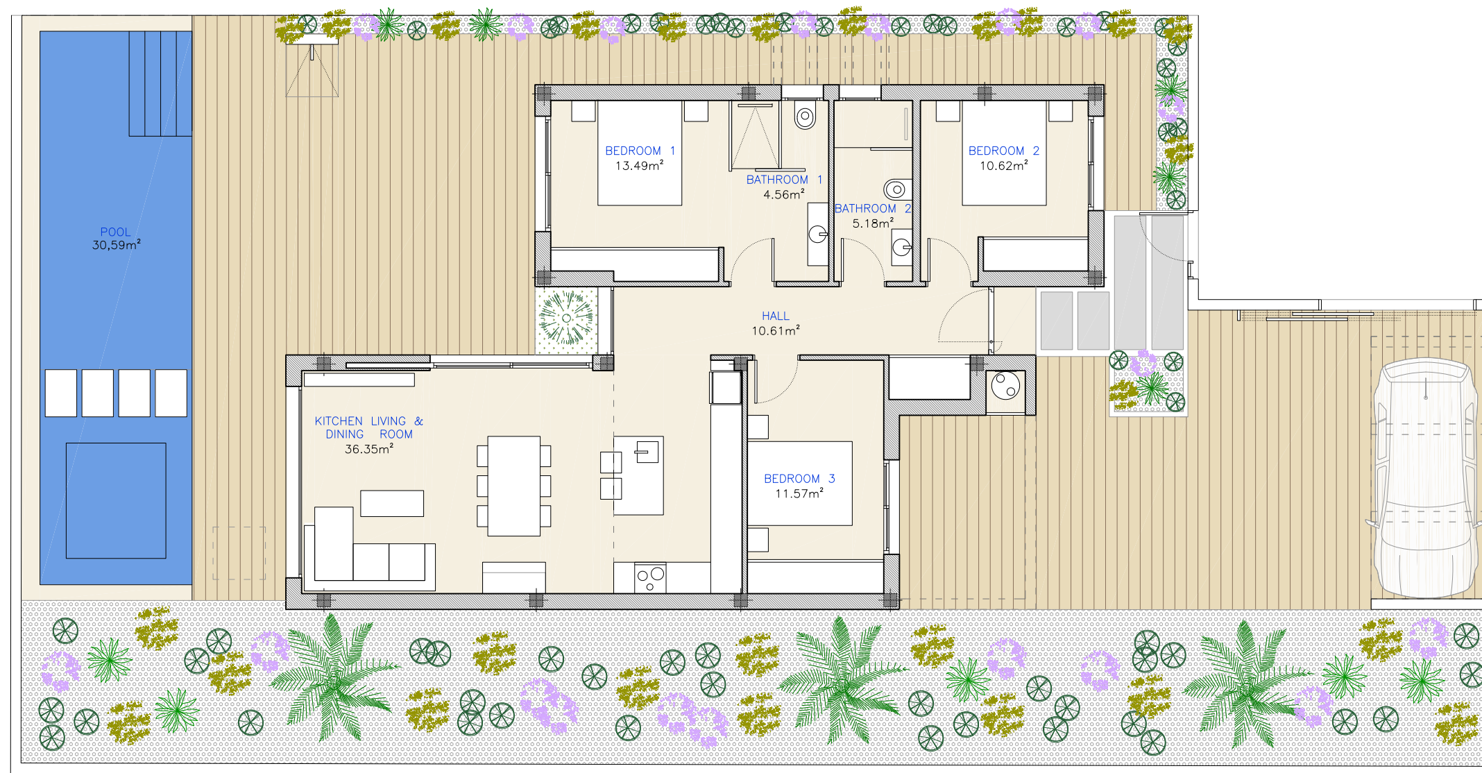
GROUND FLOOR
