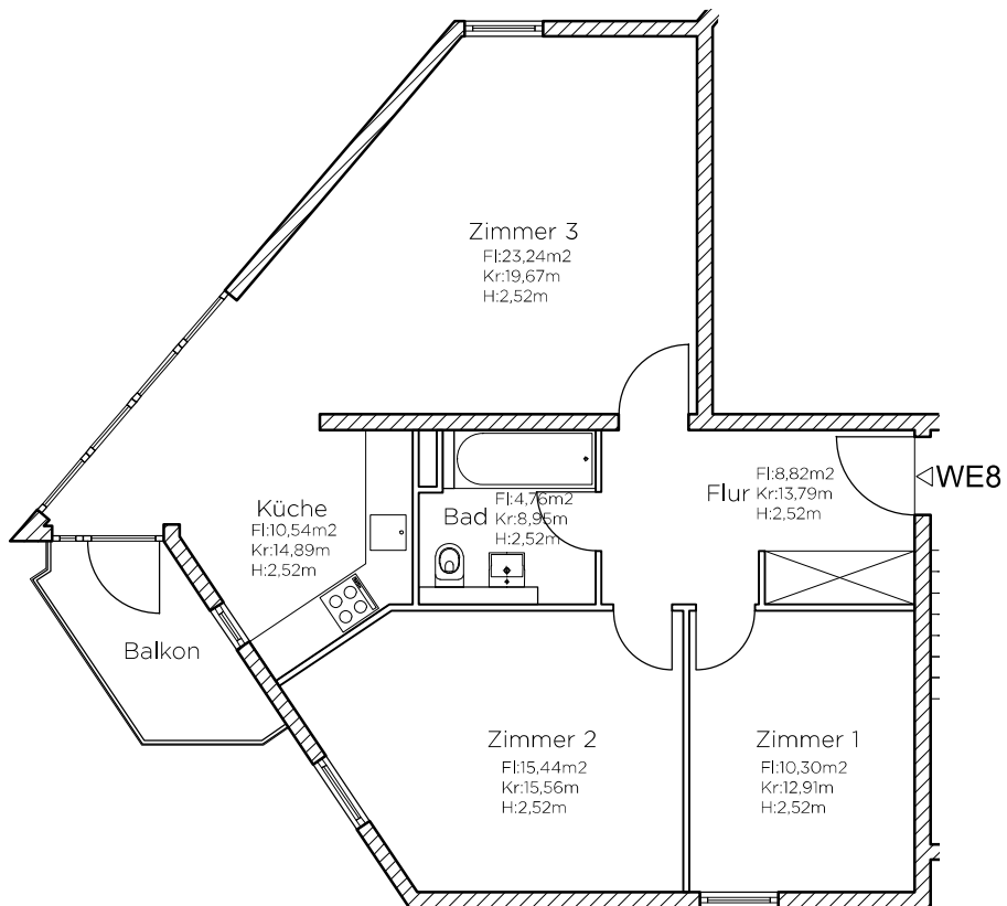
3.OG links 1:100
