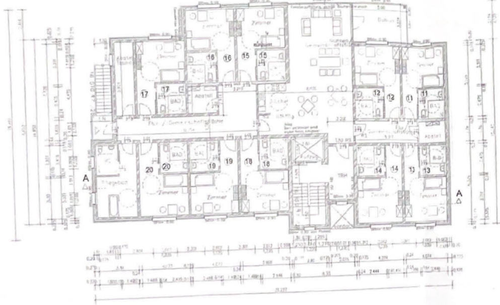
Grundriss 1.0G
