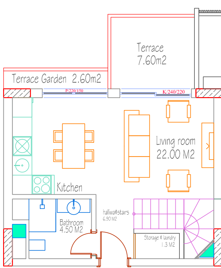
Entrance Floor Plan
