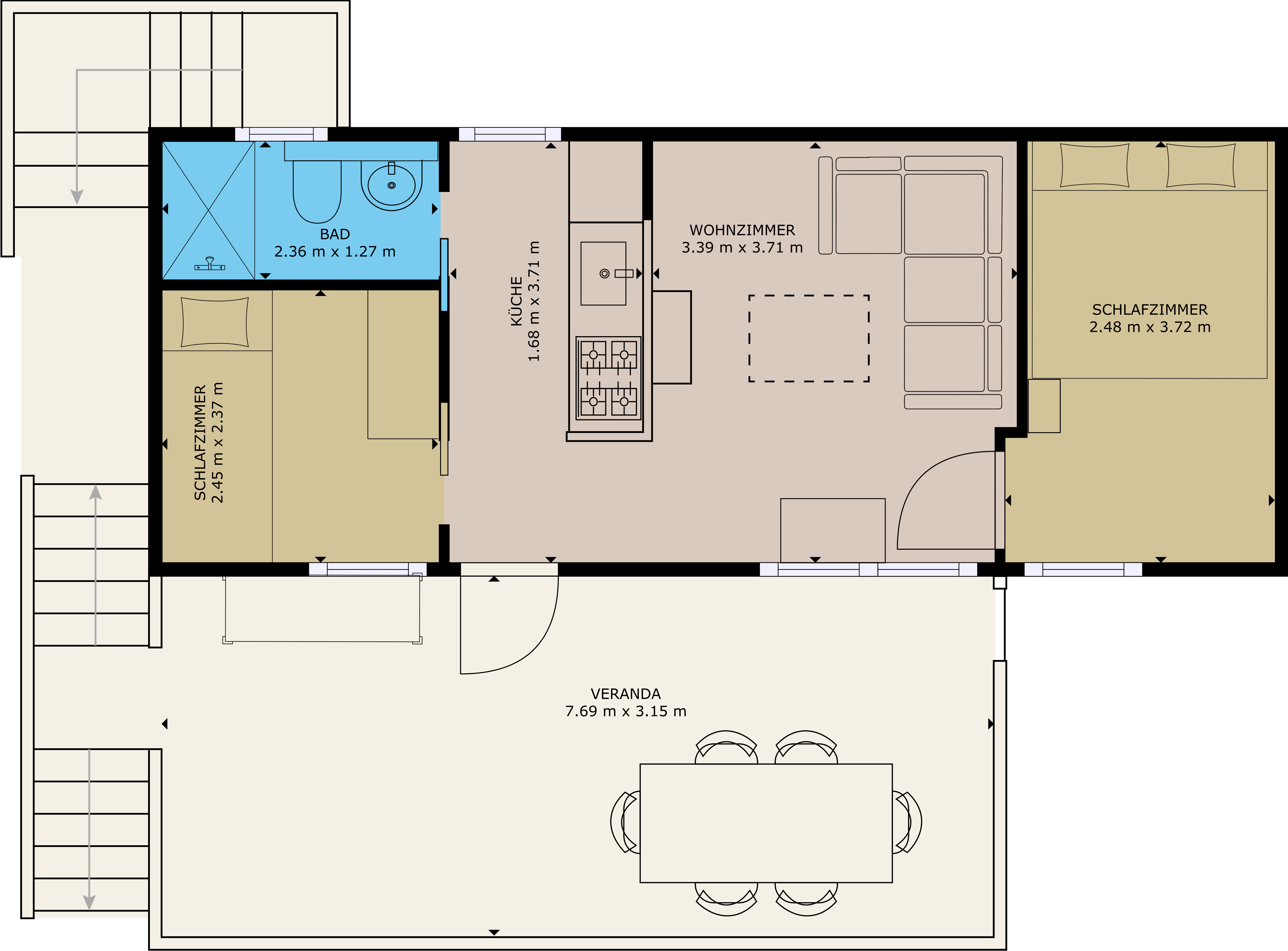
FLOOR PLAN
