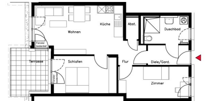
Grundriss C3
