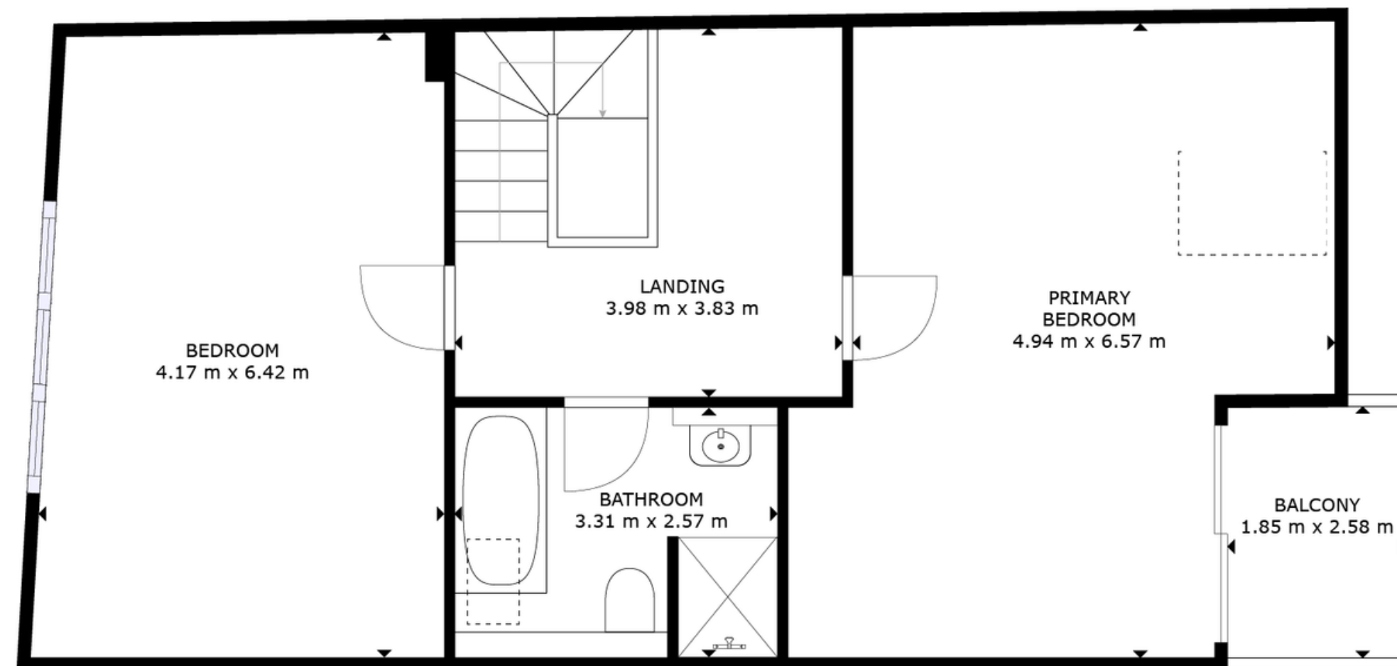
FLOOR 2
