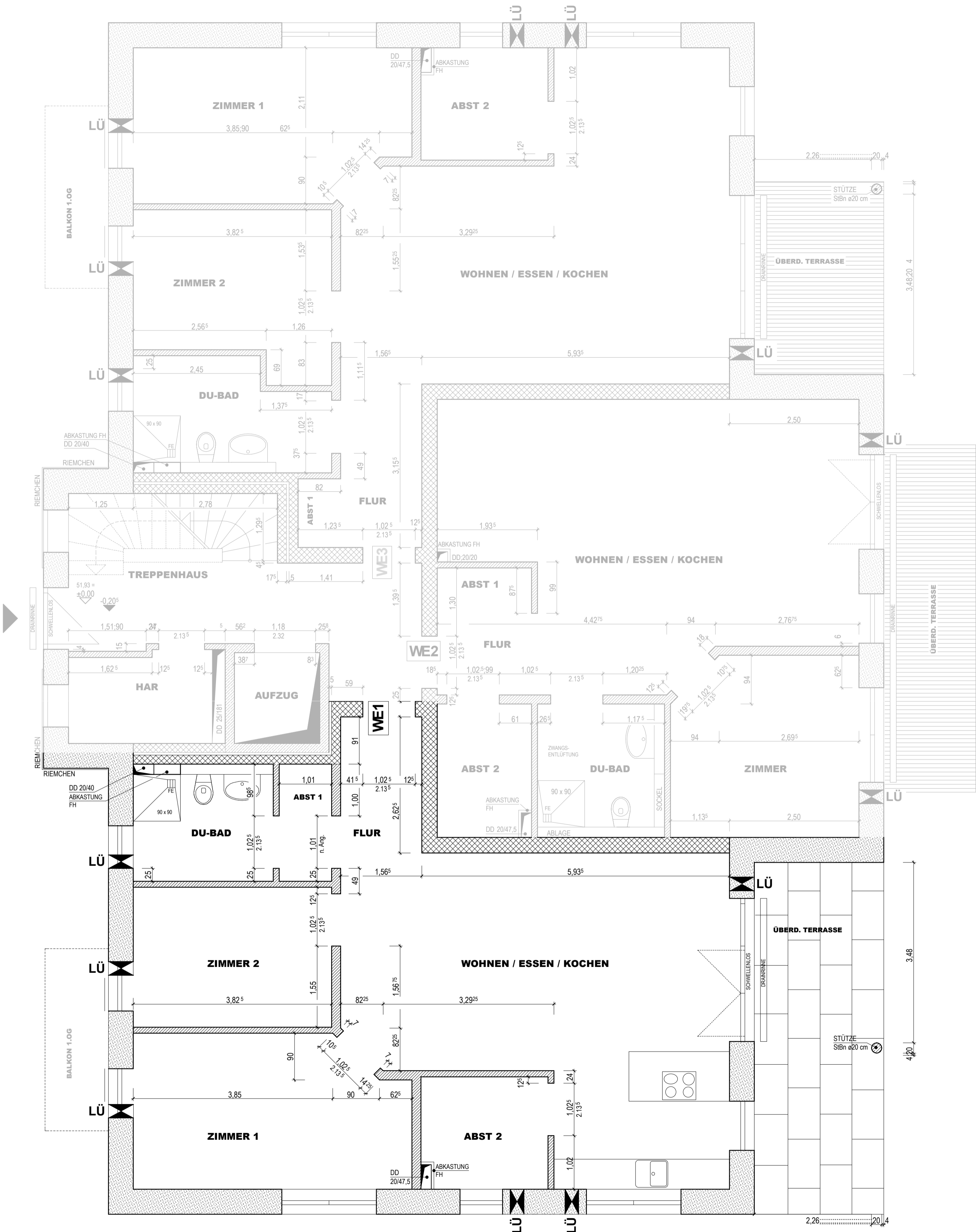
DETAIL EG M 1:50
