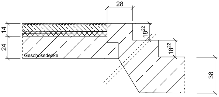
Detail Treppe OG-DG M 1:25
