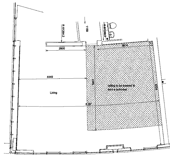
02 Reflective Ceiling Plan
