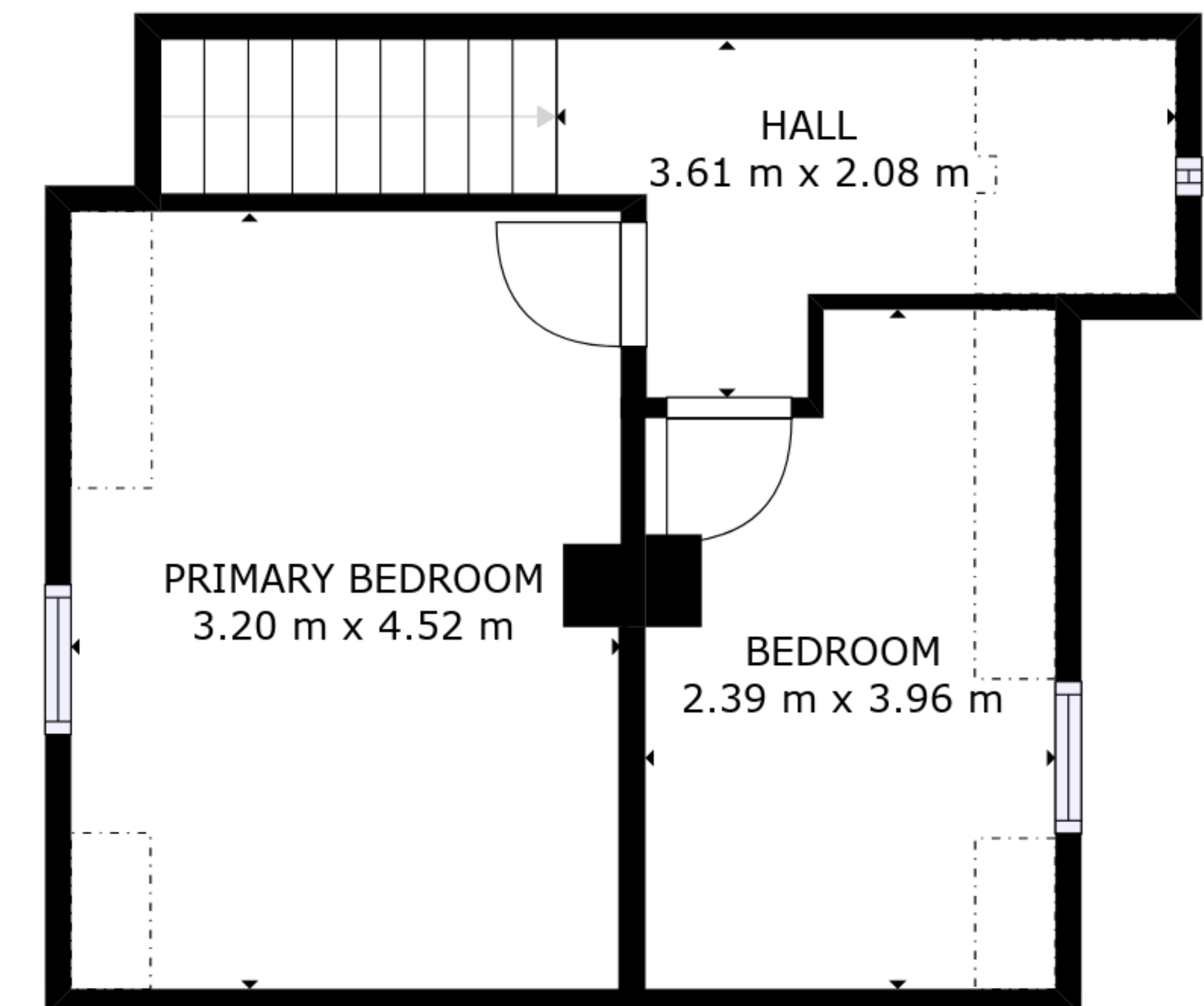
FLOOR 3
