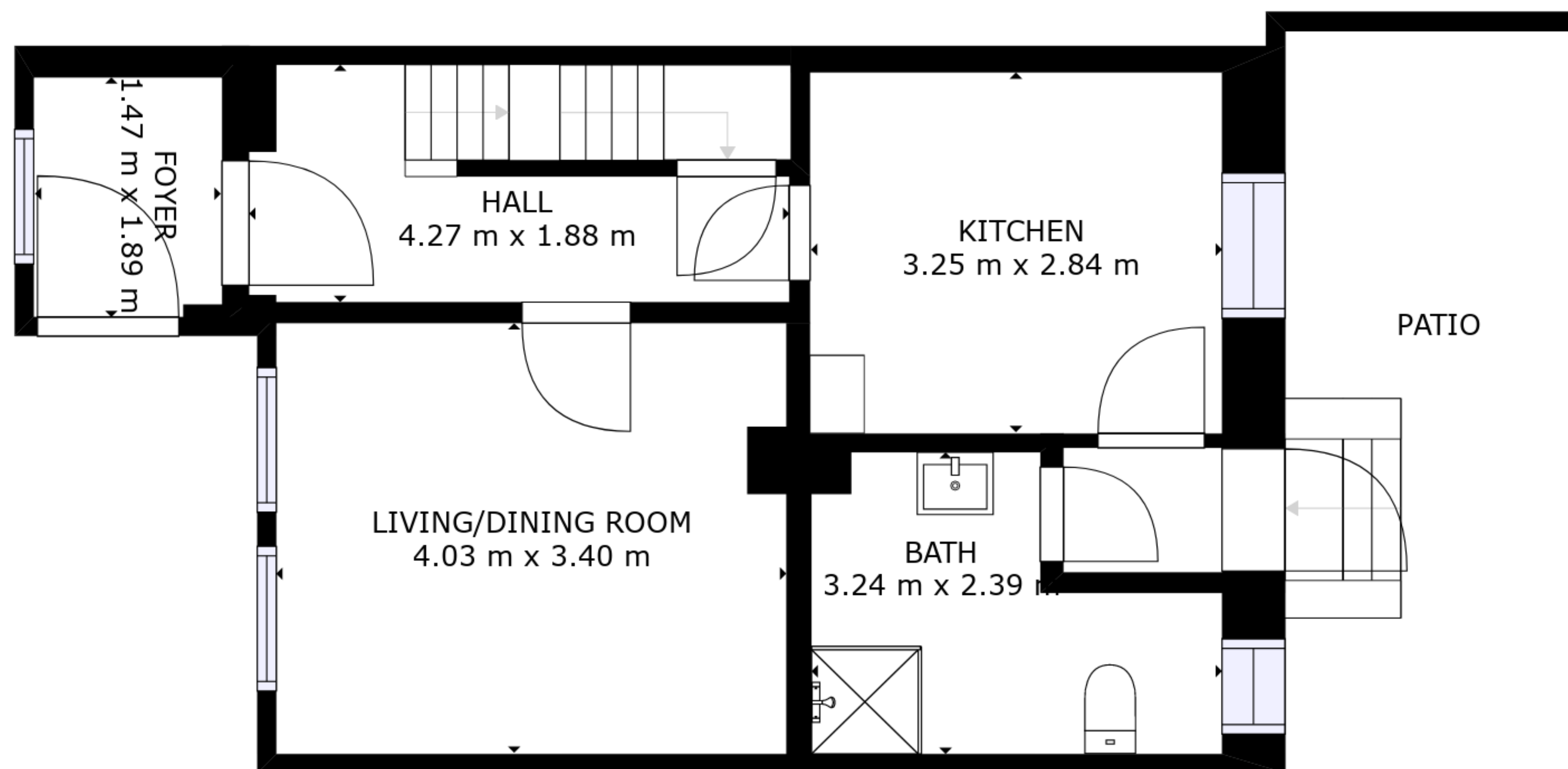
FLOOR 2
