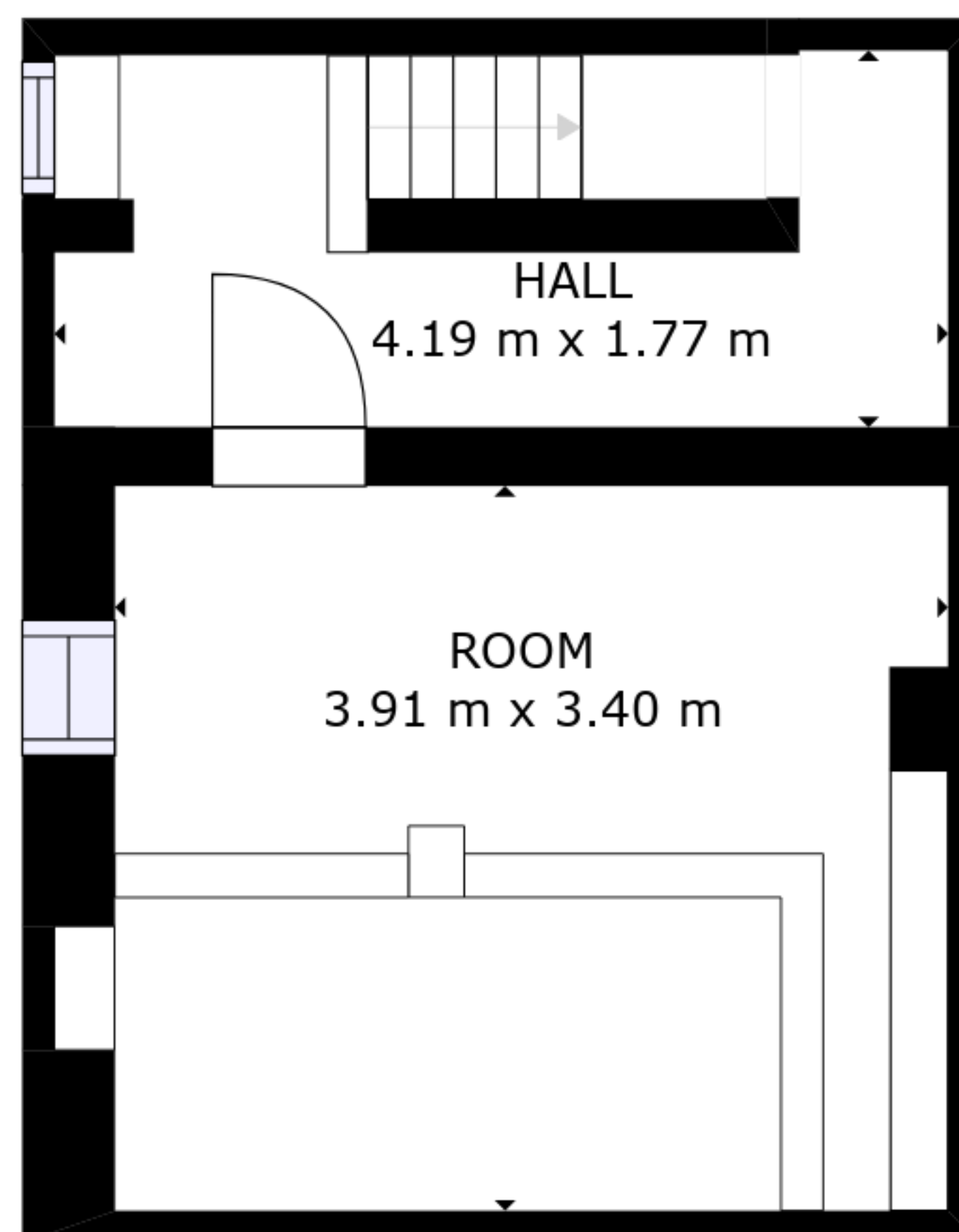
FLOOR 1
