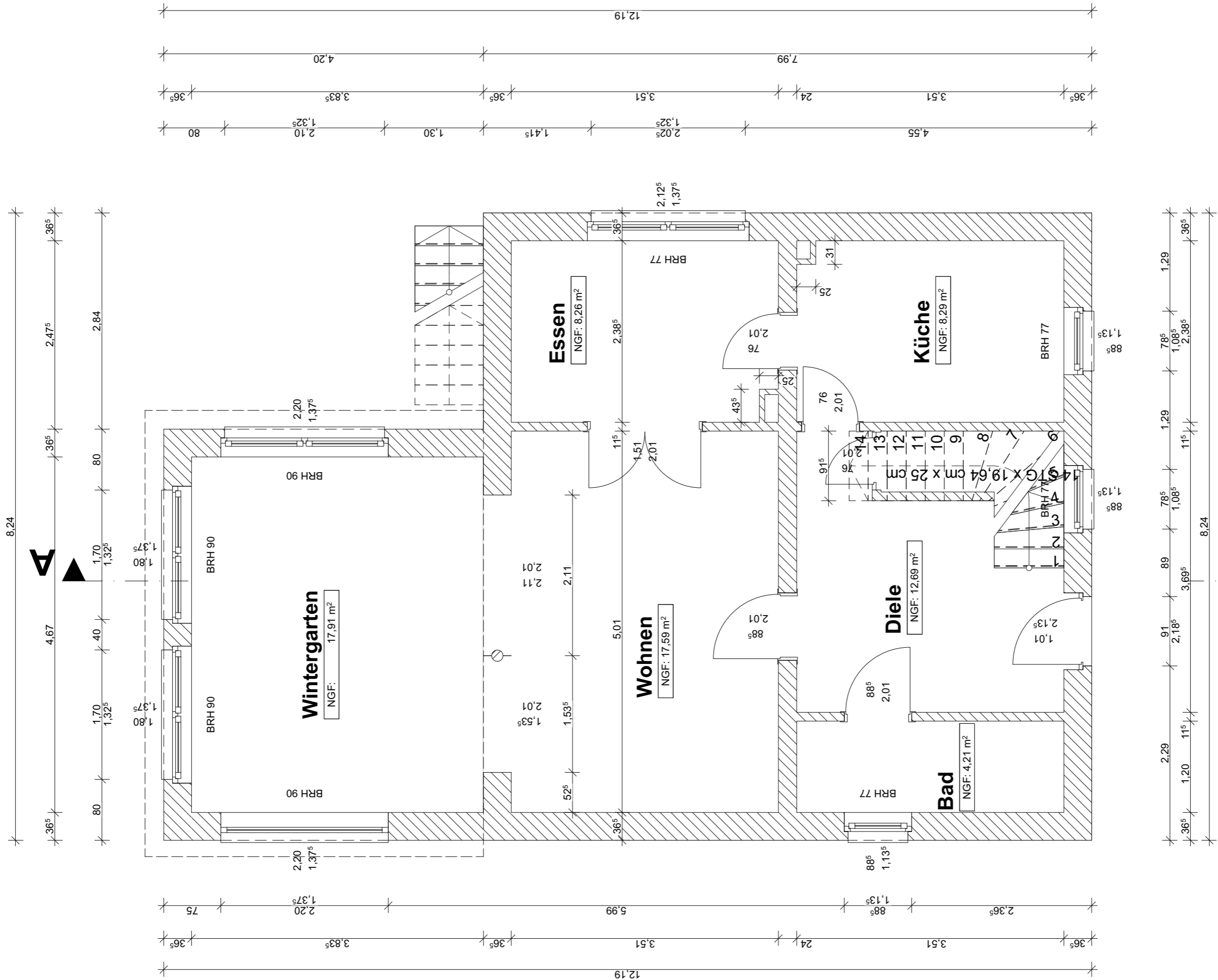
Erdgeschoss M1:50
