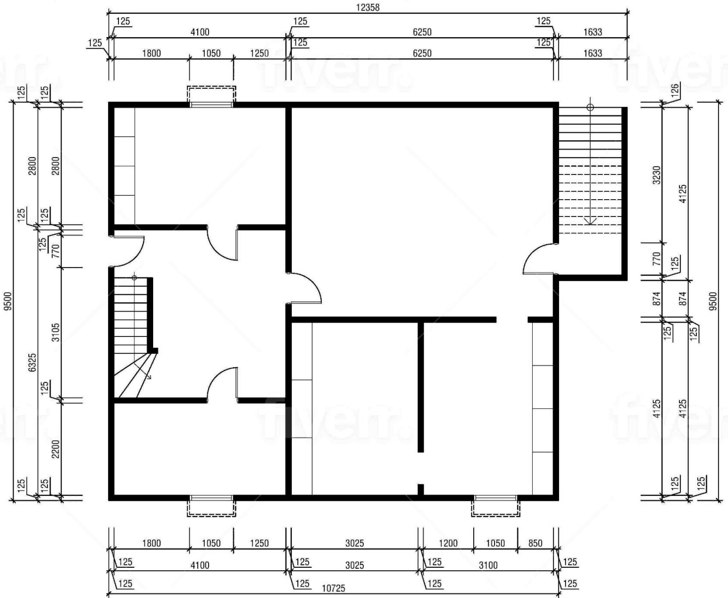
FLOOR LAYOUT PLAN SCALE A3= 1:75
